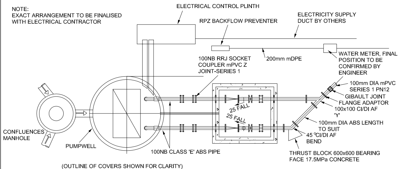
PUMPING STATION/VALVE CHAMBER PLAN
