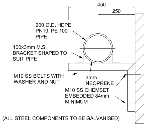
SUPPORT BRACKET FOR H.D.P.E. PIPELINK
