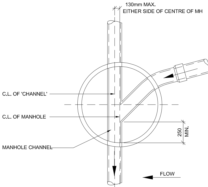
MANHOLE - PLAN VIEW
