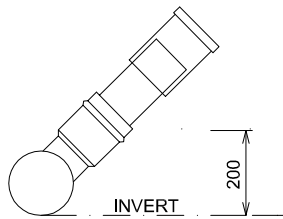
TYPICAL ELEVATION NO RAMP RISER
