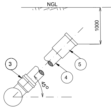
TYPICAL ELEVATION RAMP RISER
