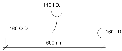
TYPE B - LONDON JUNCTION
