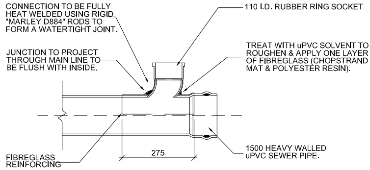
TYPICAL DETAIL - uPVC LONDON JUNCTION
