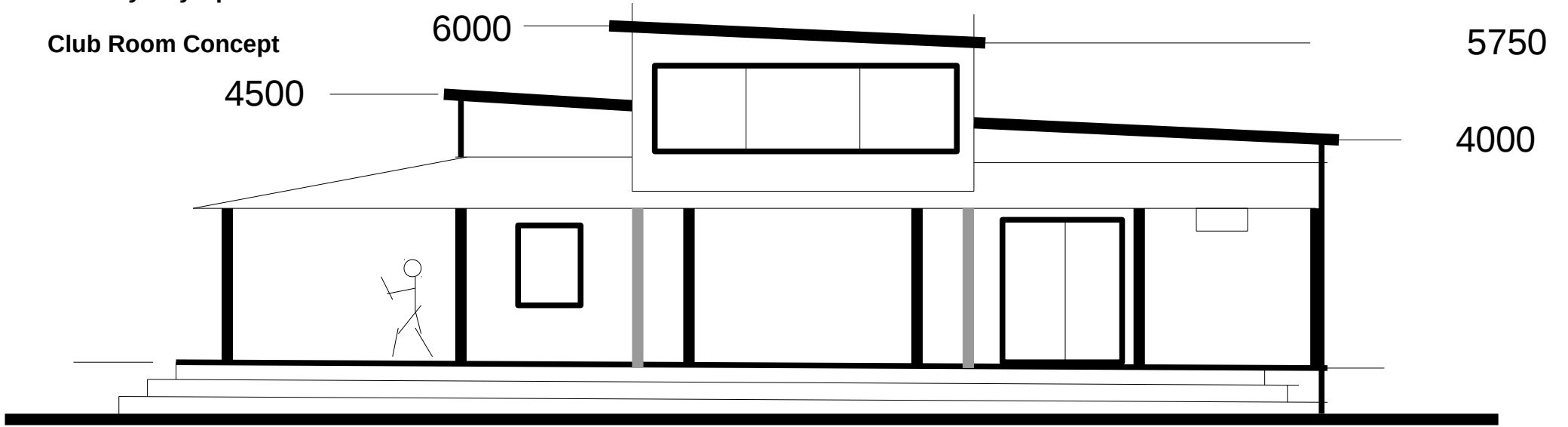
South Elevation
